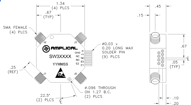
Figure 1 Mechanical Outline:
