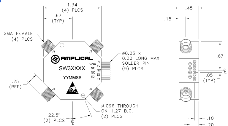
Figure 1 Mechanical Outline:
